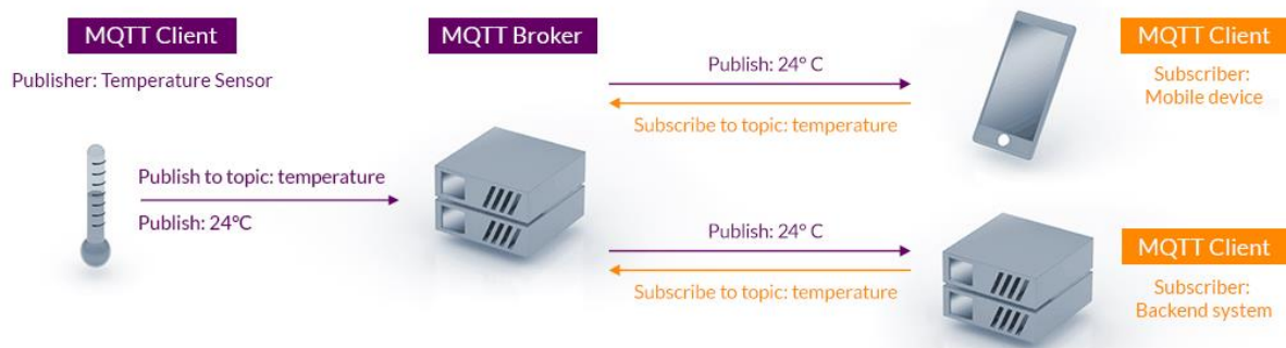
Figure 13: MQTT simplified architecture overview. 78
